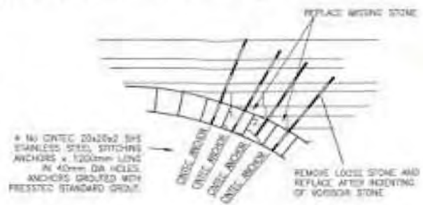
PART ELEVATION OF VOUSSOIRS/SPANREL FACE
