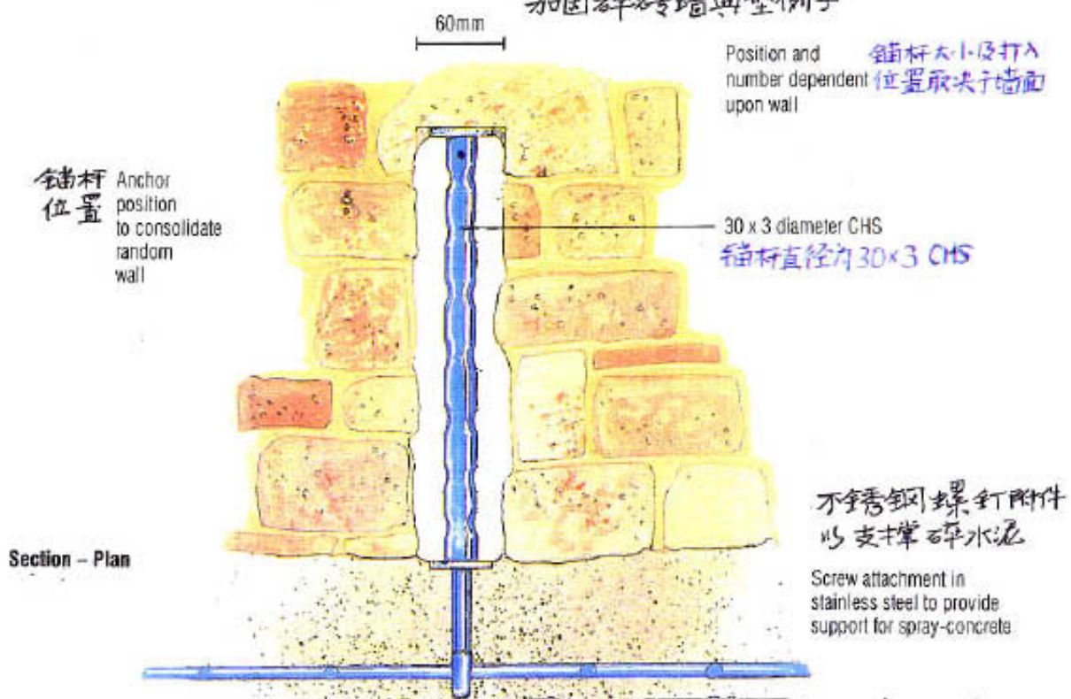
Typical Consolidation of Random Rubble Wall
